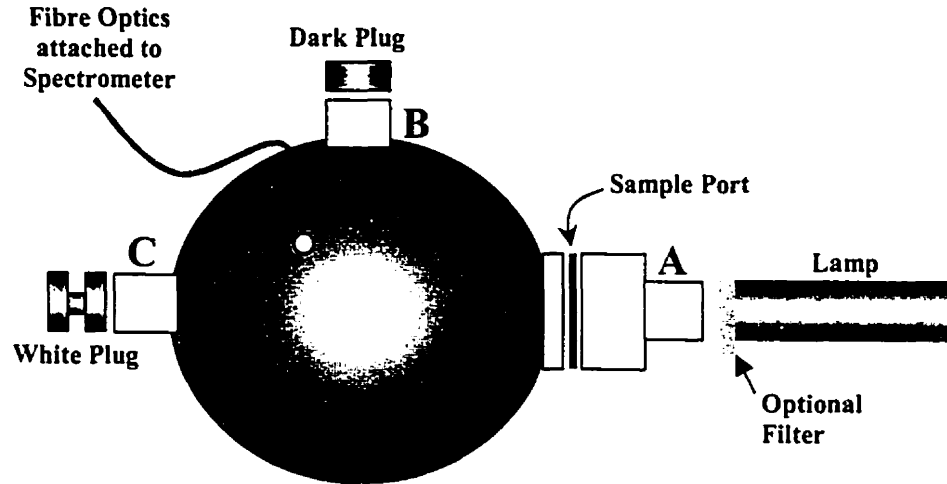
Figure 3.2. Schematic view of the Li-Cor 1800 integrating sphere coated internally with BaSO 4 , coupled to the Ocean Optics spectrometer. Ports A, B, and C enable the exchange of white and dark plugs as well as the light source. The optional long-pass filter placed at the exit aperture of the light source enables measurements of reflectance and transmittance at \lambda > 700 nm while suppressing the fluorescence signal.
