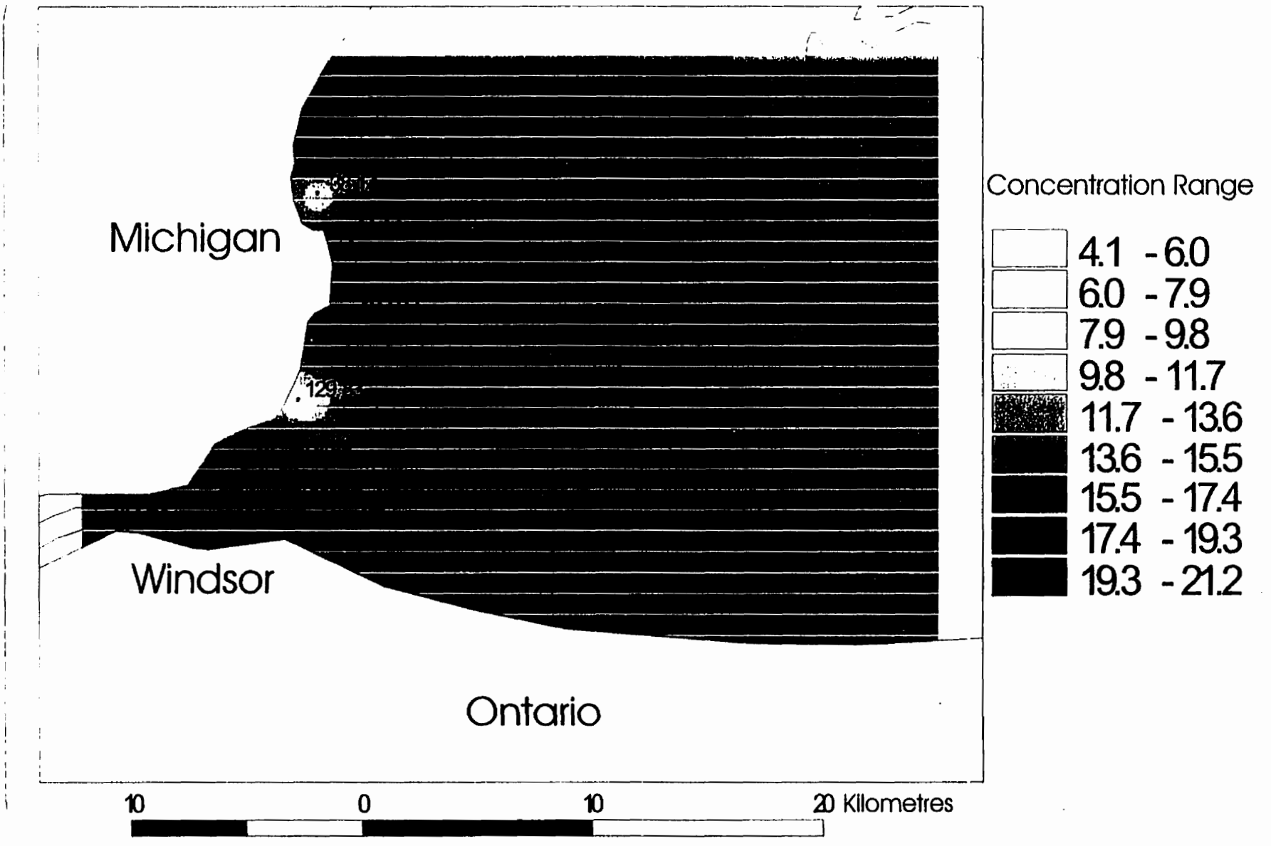
Figure 8.4: GIS Generated Map Showing the Distribution of Mn (ppm) in Shells of Dreissena polymorpha .
