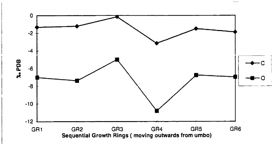
Figure 7.11: Distribution of \delta^{13}\text{C} and \delta^{18}\text{O} in growth rings of shell 17 (Detroit River Mouth).
