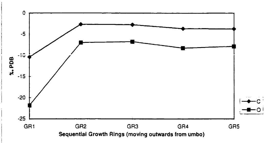
Figure 7.7: Distribution of \delta^{13}\text{C} and \delta^{18}\text{O} in growth rings of shell 8 (Grosse Pointe)
